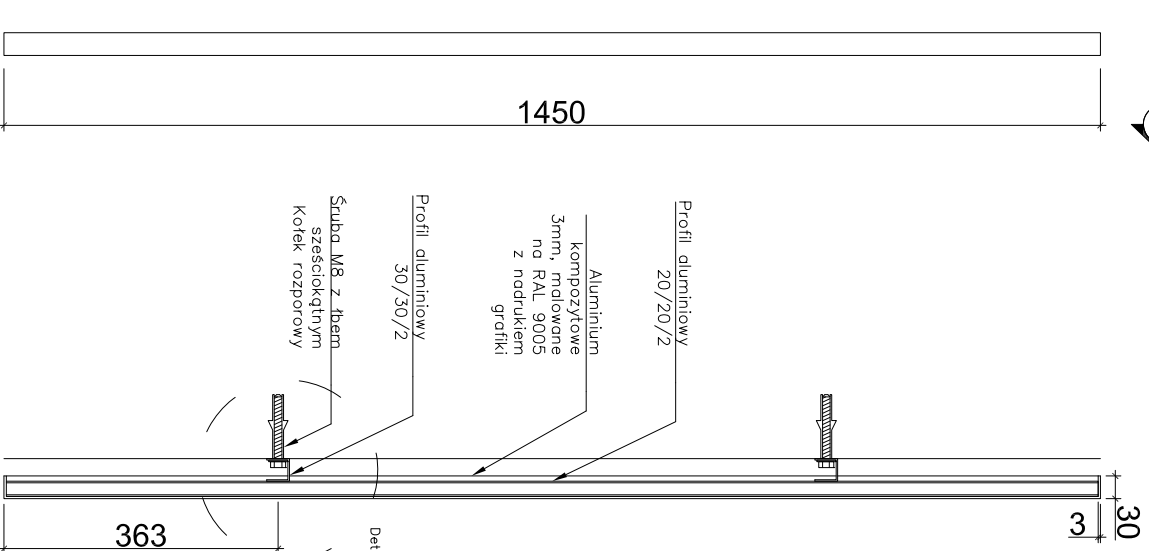
4 Widok B 1:10 @ A3
